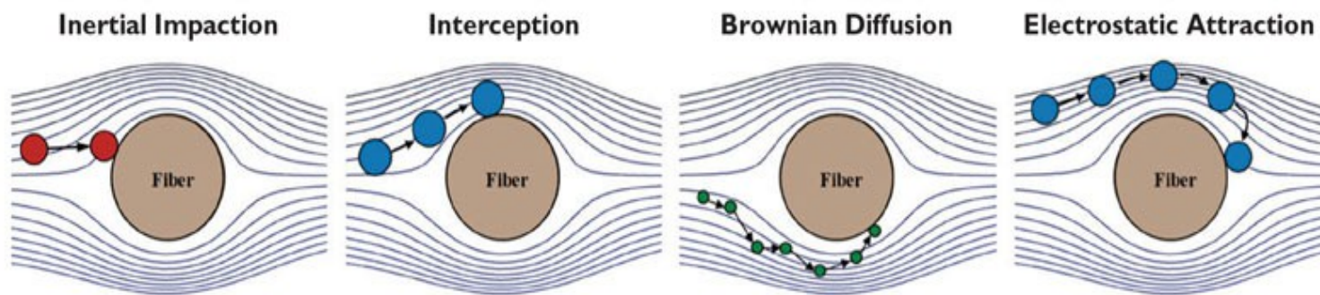
Figure 1: Filtration mechanisms
